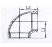
ELBOW 90° F + F
